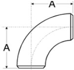
Dimensions (based on ASME/ANSI B16.9) and example weights for long radius elbows
